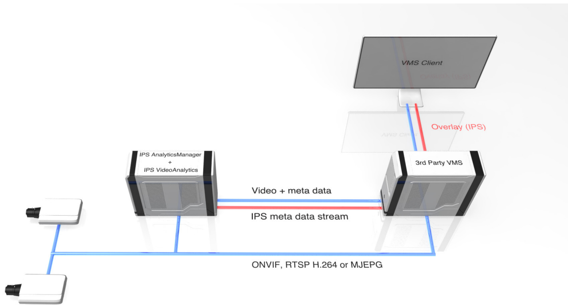
Above: Possible option for the integration of IPS VideoAnalytics into 3rd party video management systems via IPS AnalyticsManager.
