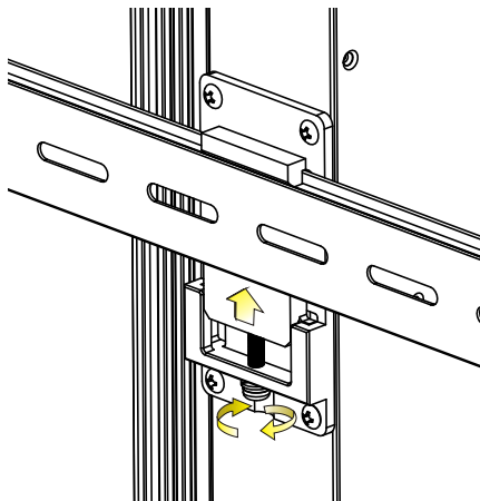
Figure 3-19: Secure the Mounting Bracket
