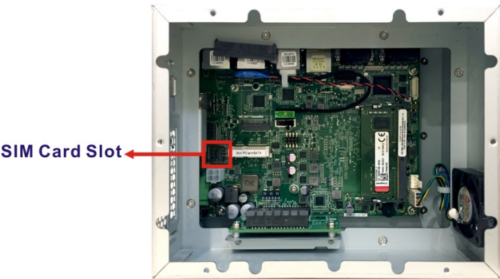
Figure 3-7: Unlock SIM Card Slot Cover
