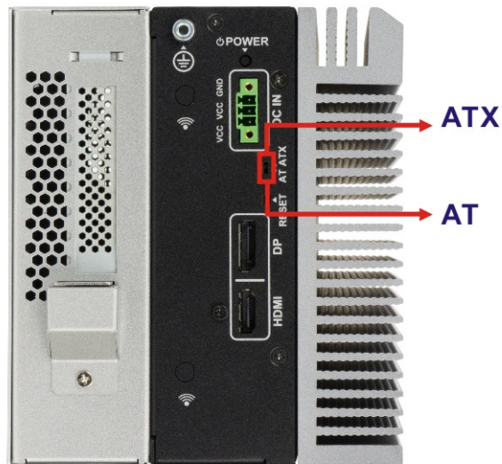
Figure 3-15: AT/ATX Switch Location
