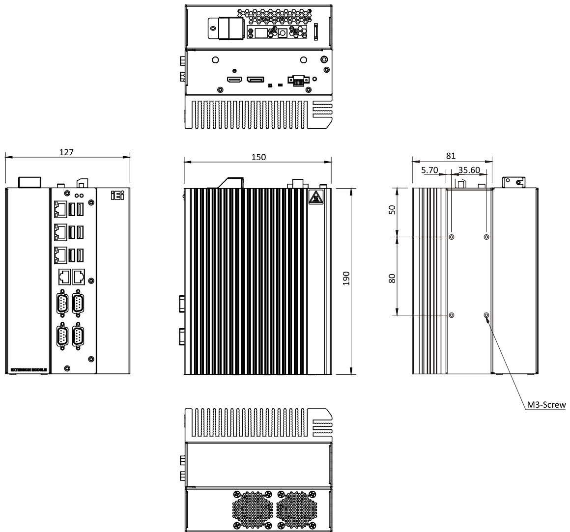
Figure 1-5: DRPC-230-ULT5-i5/8G Dimensions (mm)
