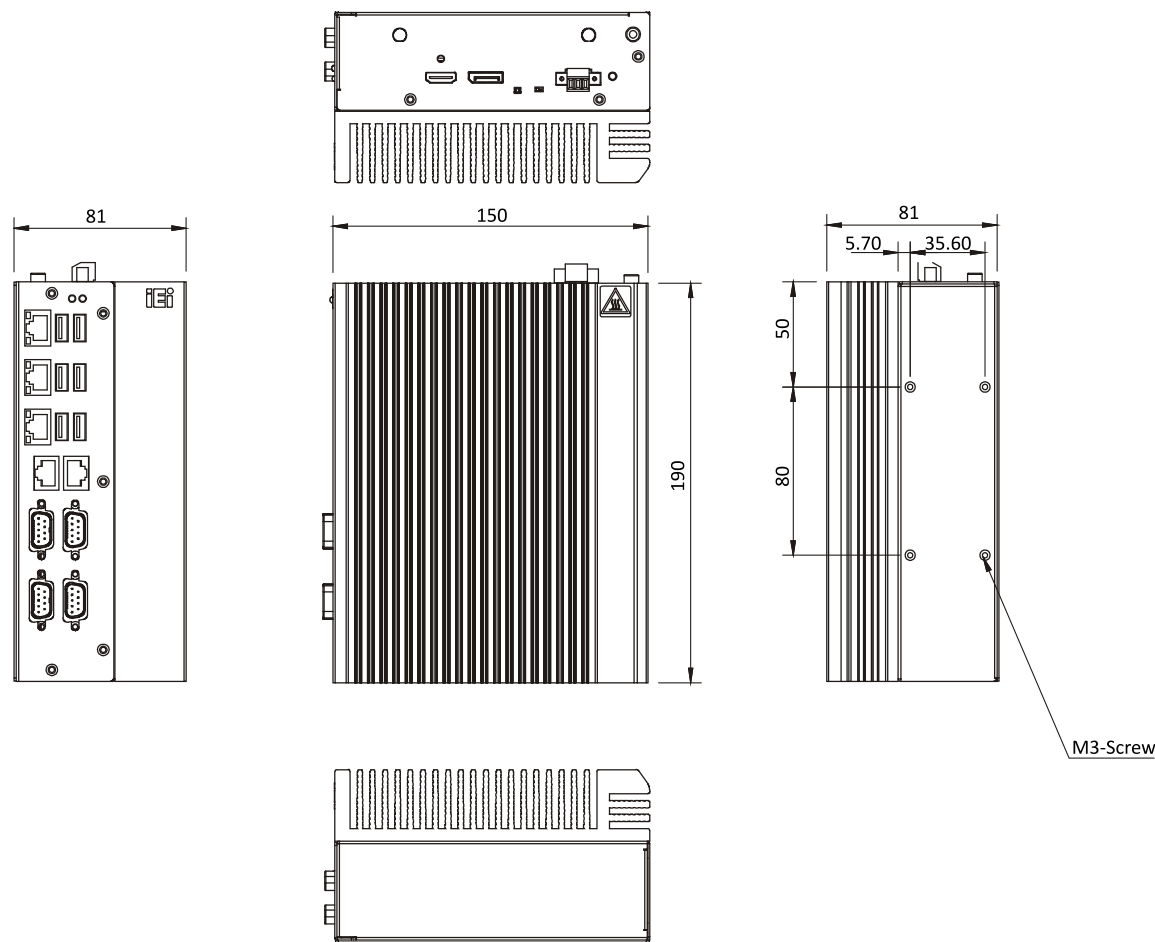
Figure 1-4: DRPC-230-ULT5-i5/8G/S & DRPC-230-ULT5-C/8G/S Dimensions (mm)
