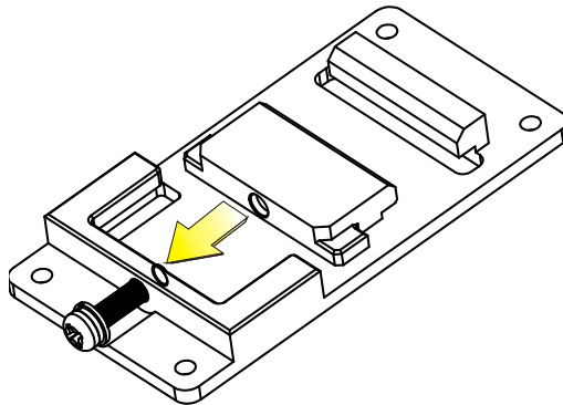
Figure 3-16: DIN Rail Mounting Bracket Preparation
