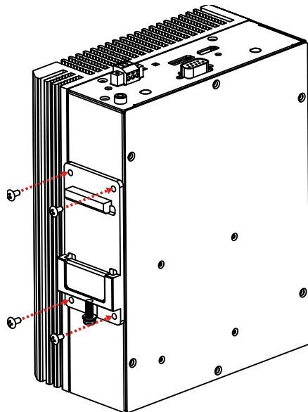
Figure 3-17: DIN Rail Mounting Bracket Installation
