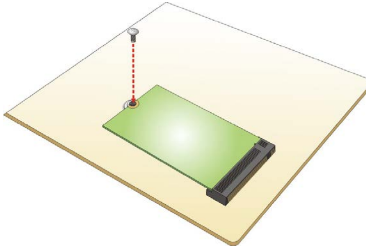
Figure 3-13: Securing the M.2 Module
