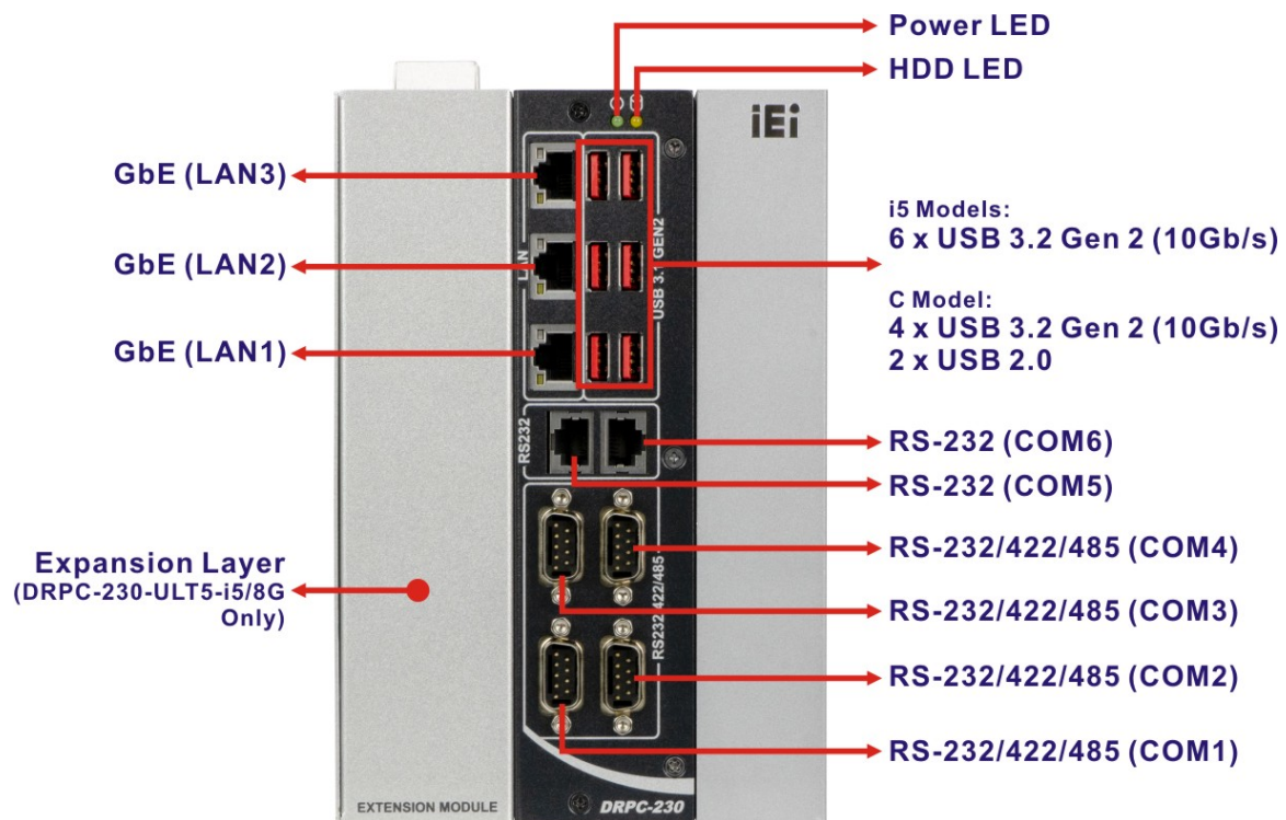
Figure 1-2: Front Panel
