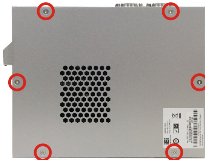
Figure 3-1: Internal Access Panel Retention Screws
