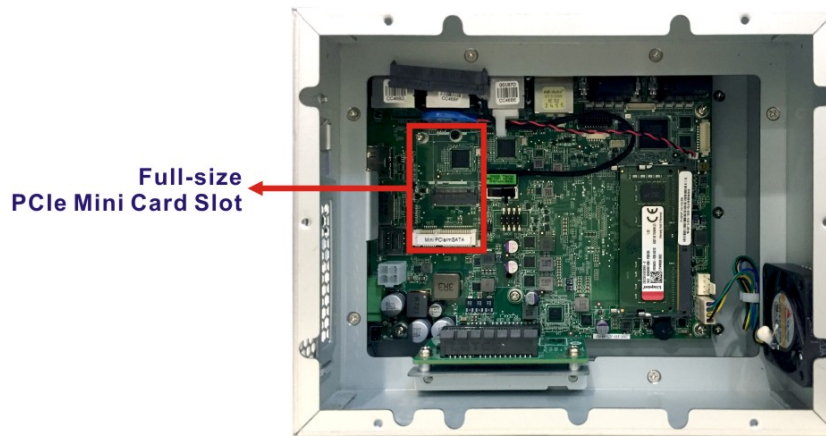
Figure 3-3: PCIe Mini Slot Location
