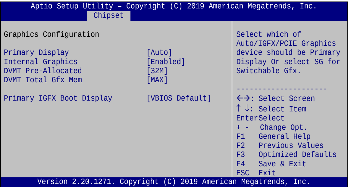
BIOS Menu 23: Graphics Configuration
