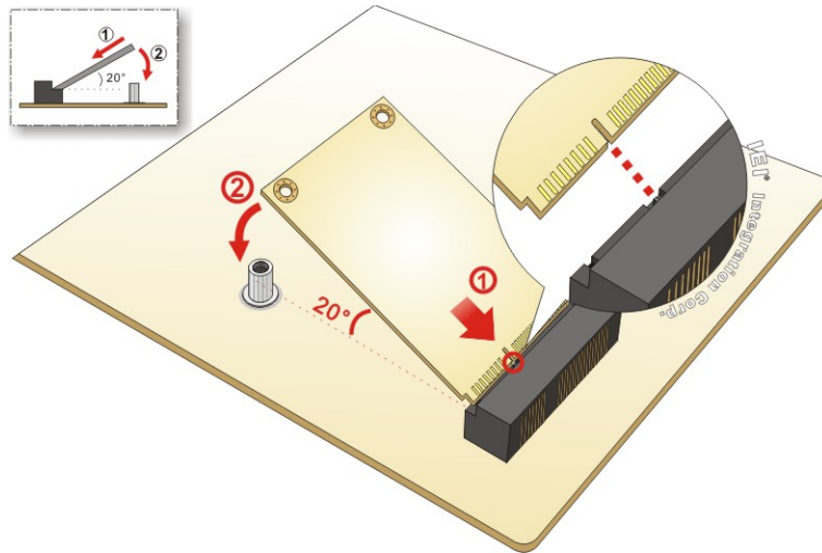
Figure 3-5: Inserting the PCIe Mini Card into the Slot at an Angle
