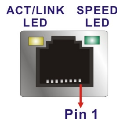
Figure 3-14: RJ-45 Ethernet Connector
