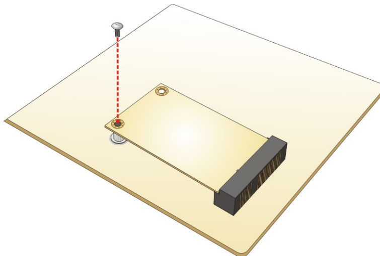
Figure 3-6: Securing the PCIe Mini Card
