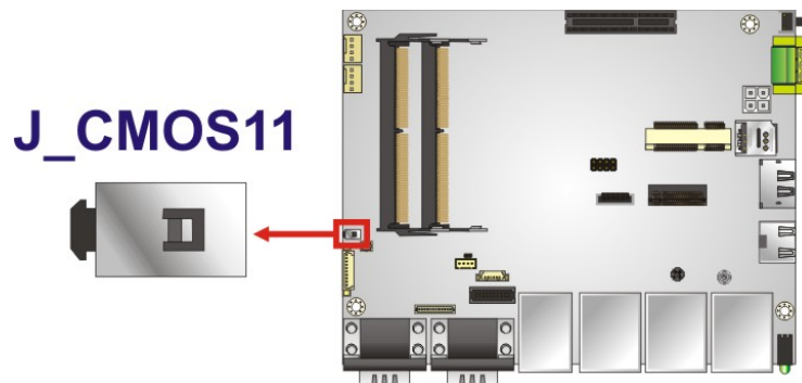
Figure 4-1: Clear CMOS Button Location
