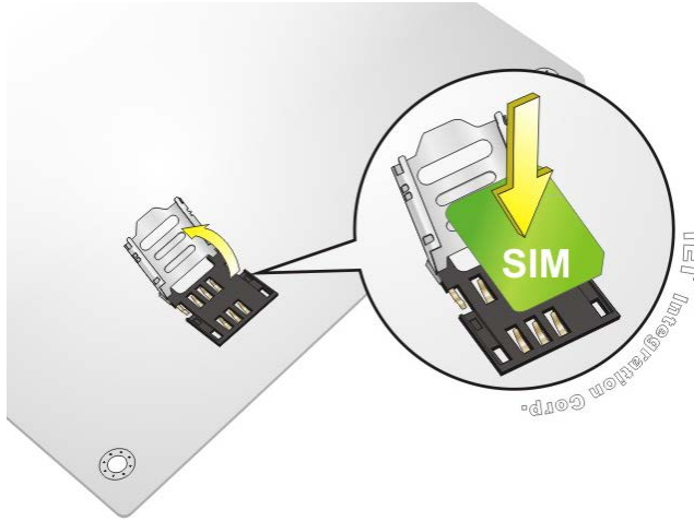
Figure 3-9: SIM Card Installation
