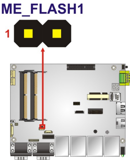
Figure 4-2: ME Override Jumper Location
