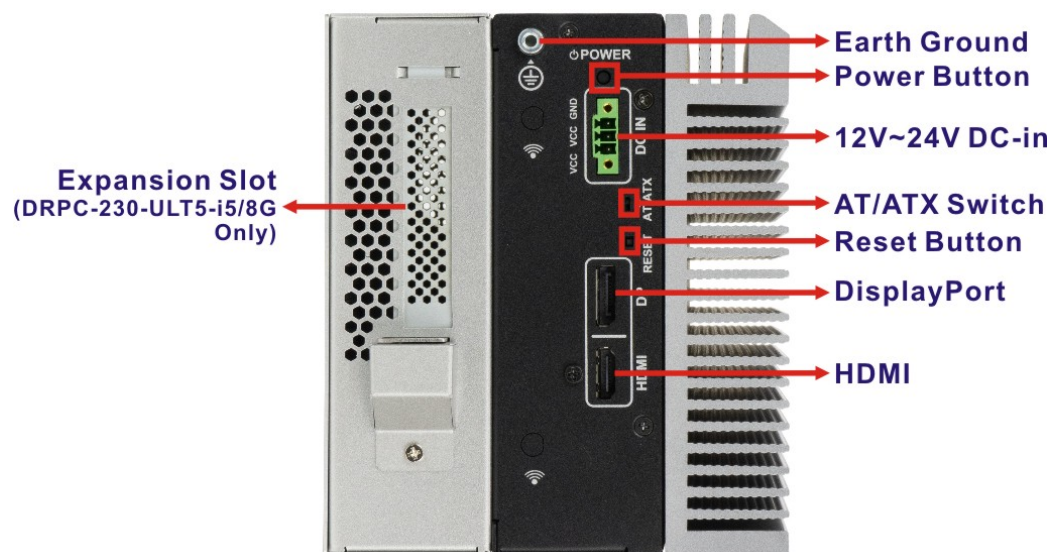
Figure 1-3: Top Panel
