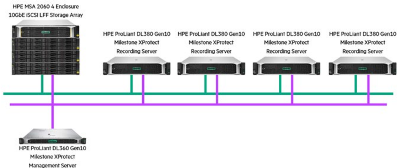
Figure 3. High-level architectural view of the verification setup
