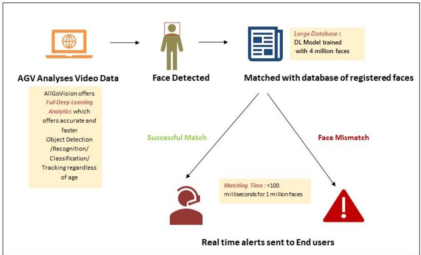
AllGoVision Face Recognition Flow
