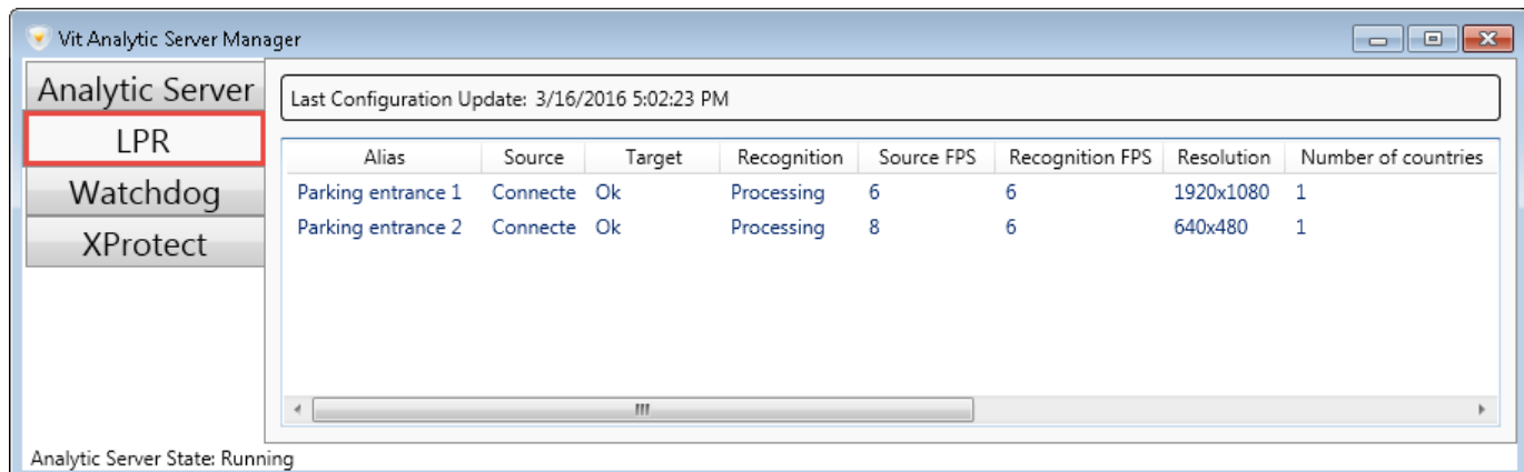
Figure 17: Monitoring feature for active recognition channels, Analytic Server manager
