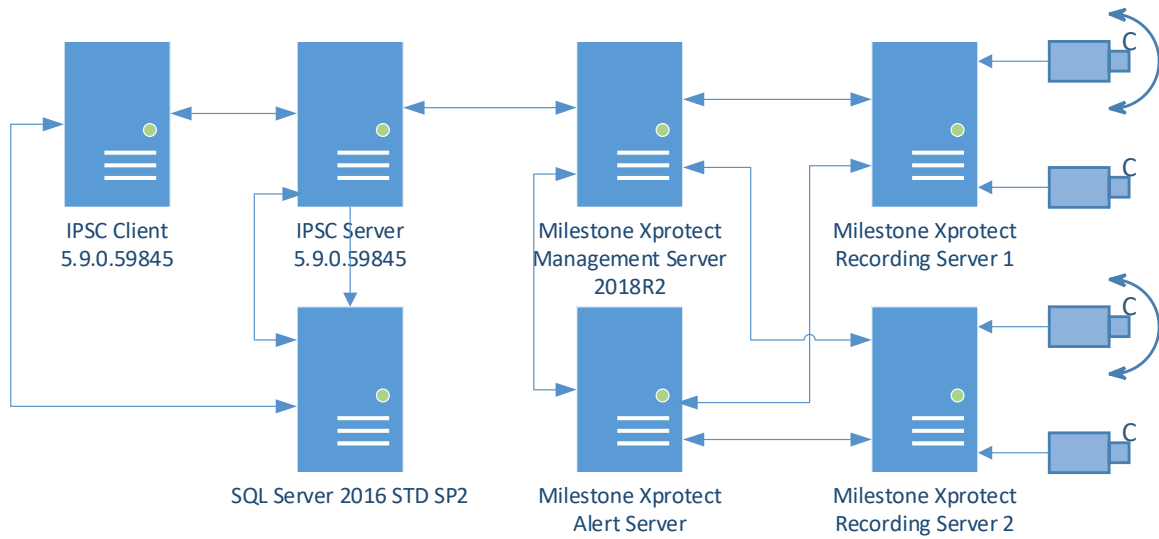
Figure 1 Milestone IPSC Schematics
