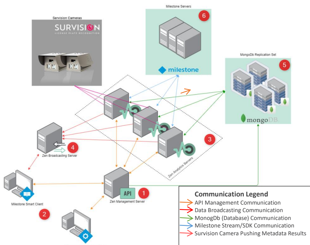
Figure 1 - Servers Diagram
